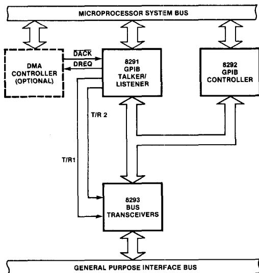
Figure 1. 8291, 8292, 8293 Block Diagram
