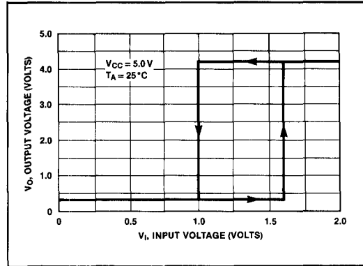
Typical Receiver Hysteresis Characteristics
