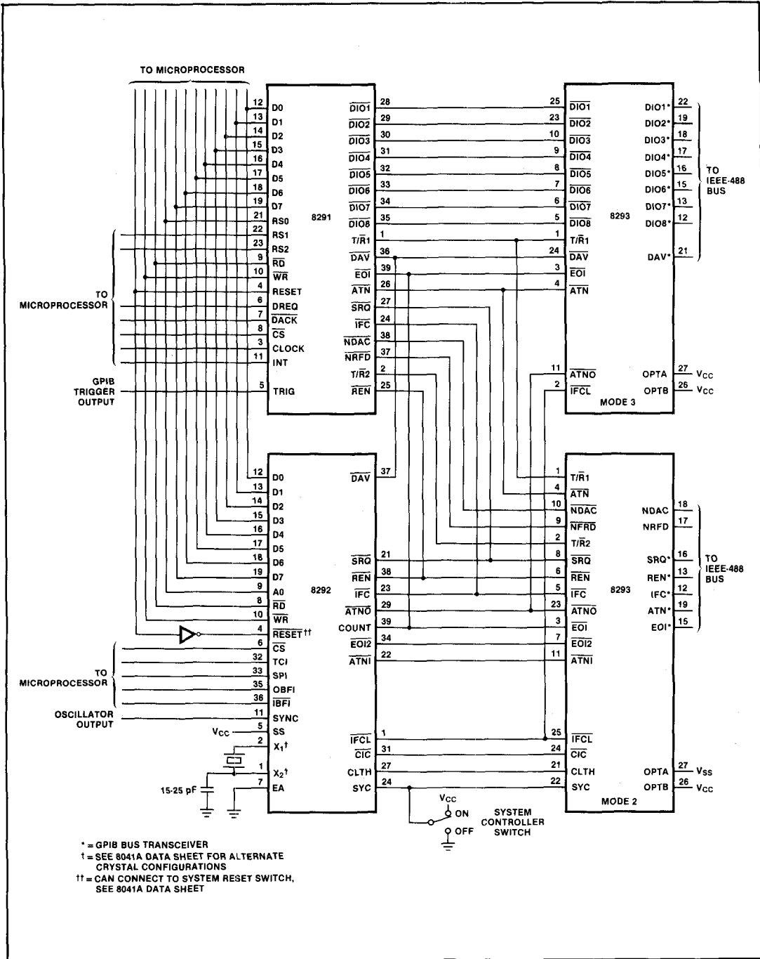
Figure 10. 8291, 8292, and 8293 System Configuration
