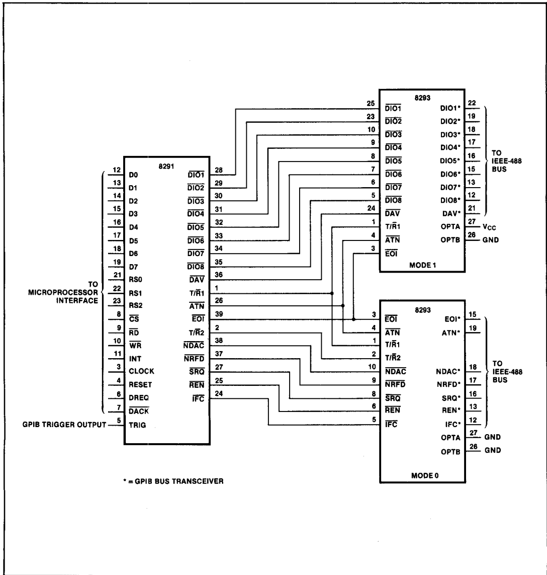
Figure 9. 8291 and 8293 System Configuration
