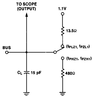
Send/Receive Input to Bus Output (Driver)
