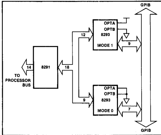
Figure 3. Talker/Listener Configuration
