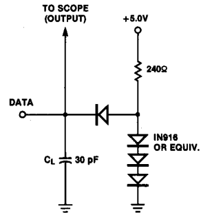
Bus Input to Data Output (Receiver)
