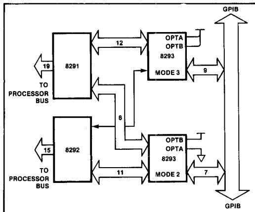
Figure 4. Talker/Listener/Controller Configuration
