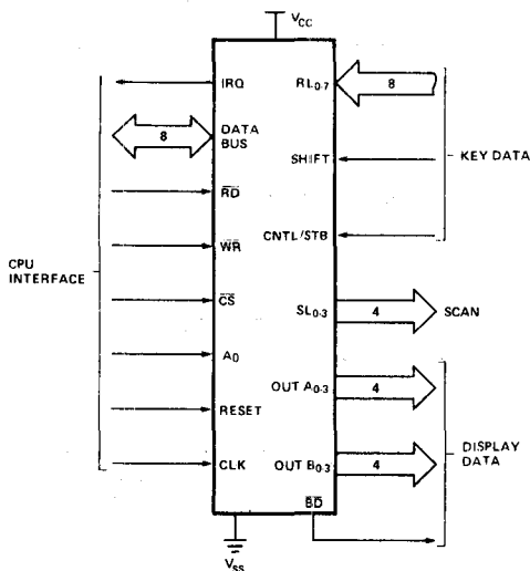
Figure 1. Logic Symbol
